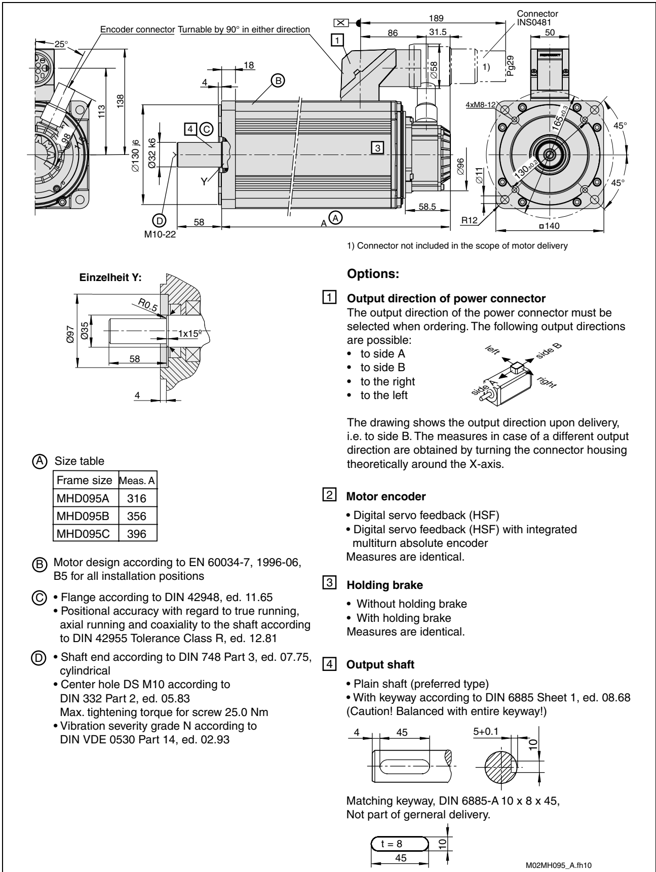
Fig. 10-16: Dimensional details of MHD095.-...-N
